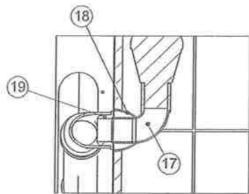
SECTION F-F SCALE 1 : 5
